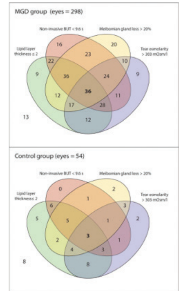
FIGURE 3. Venn diagram analysis of both MGD and control groups. Cutoff values of non-invasive BUT, meibomian gland loss, lipid layer thickness, and tear osmolarity were determined from ROC curves.
